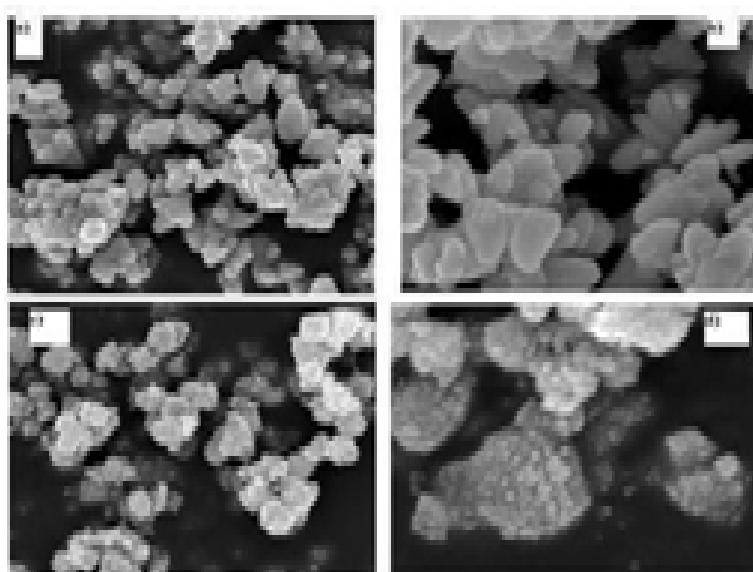
Figure 2. 2a) Micrograph of chemically synthesized ZnO particles at lower magnification; 2b) Higher magnification green synthesized ZnO particles at; 2c: Lower magnification; 2d: Higher magnification.
