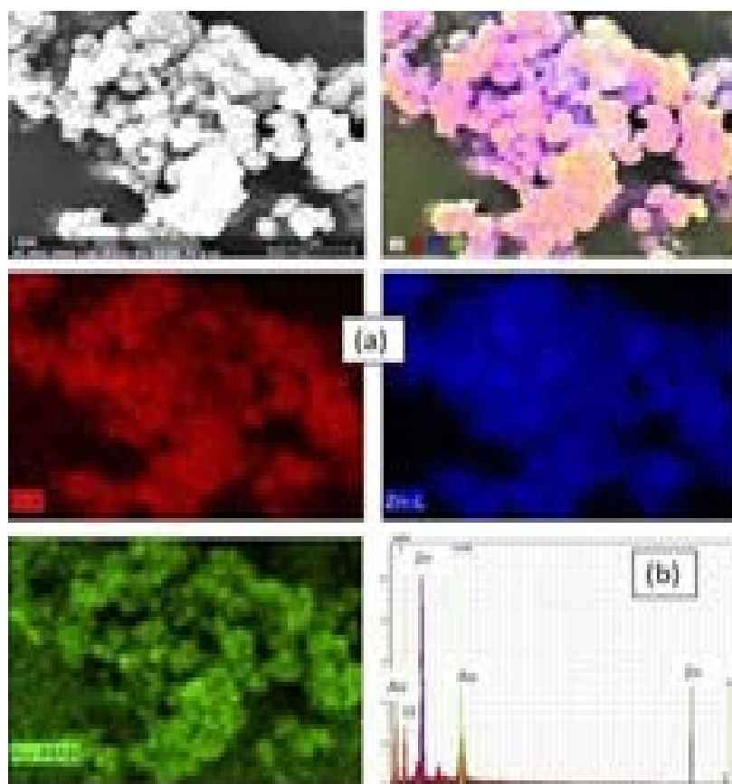
Figure 3. 3a) Elementary mapping of 500°C calcined chemically synthesized ZnO powder showing the distribution of elements such as O and Zn; 3b) EDX spectra of green synthesized ZnO powder.
