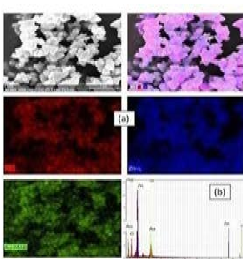
Figure 4. 4a) Elementary mapping of 500°C calcined green synthesized ZnO powder showing distribution of elements such as O and Zn; 4b) EDX spectra of green synthesized ZnO powder.
