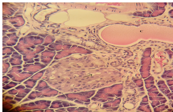
Figure 3. Pancreas of diabetic rats showing congestion(C) and slight vacuolation of islet's of Langerhans cells (arrow). (H & E stain, 400X).
