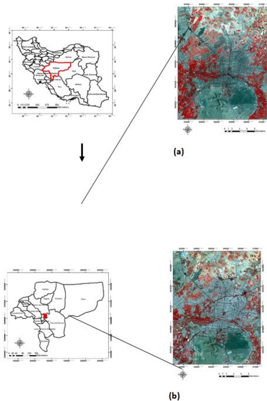
Figure 1. False color composite images demonstrating the location of the study area across Isfahan Province and its spatial dynamics between (a) 1998 and (b) 2014.
