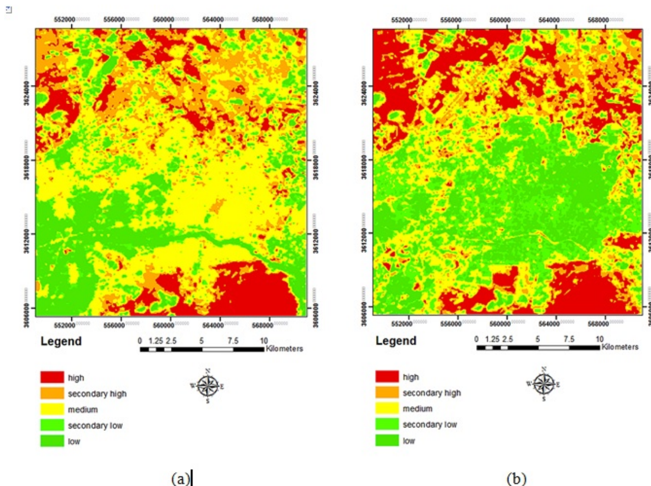
Figure 4. Classified land surface temperature layers for (a) 1998 and (b) 2014 node years.
