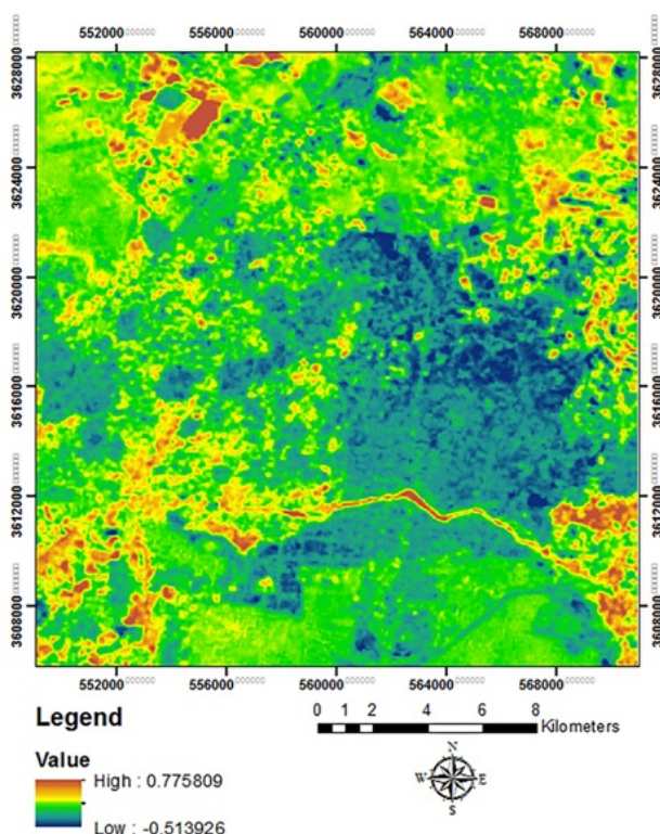
Figure 6. Pixel- based spatiotemporal dynamics of land surface temperature in Isfahan Metropolitan Area during 1998-2014 time profile.
