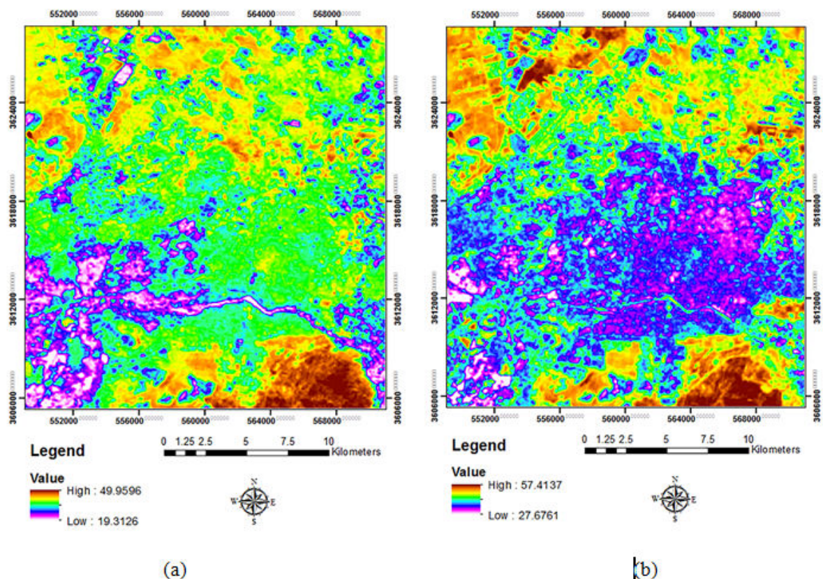
Figure 3. Land surface temperature layers for (a) 1998 and (b) 2014 node years. As it is illustrated in
