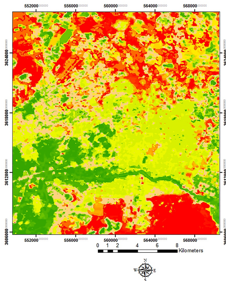
Figure 5. Cross-tabulated land surface temperature layers (1998-2014) and mutual exchanges between different temperature categories in Isfahan Metropolitan Area.
