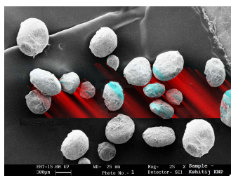
Figure 1. Microspheres with size ranging approximately from 300 to 900 µm.
