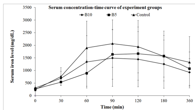
Figure 1. Serum concentration-time curve of experiment groups. The rats were administered ferrous sulphate ( 760 \text{ mg.kg}^{-1} , equivalent to 153 \text{ mg.kg}^{-1} elemental iron, 750 \mu\text{l} ) application, five minutes later, the Control group received distilled water ( 1250 \mu\text{l} ), and the bentonite groups received 5 (B5) or 10 (B10) fold of bentonite (B5, 765 \text{ mg.kg}^{-1} or B10, 1530 \text{ mg.kg}^{-1} , 1250 \mu\text{l} ) respectively. Values are means with vertical bars indicating SD. Ferrous sulphate administration caused significant increase in serum iron concentrations in Control, B5 and B10 compared to start point. There were no differences between Control, B5 and B10.
