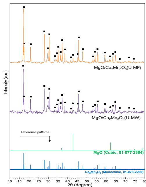
Figure 1. XRD patterns of Ca-Mn Perovskite Used in MgO Nanocatalyst: MgO/Ca 2 Mn 3 O 8 (U-MF) and MgO/Ca 2 Mn 3 O 8 (U-MW)
