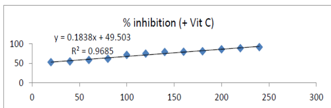
Figure 2: Calibration curve of % inhibition versus concentration (µg/ml) for Vitamin C standards
