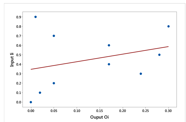
Figure 6. Input-based correlation mapping as P(O i =c 1 |I j =c 2 ).
