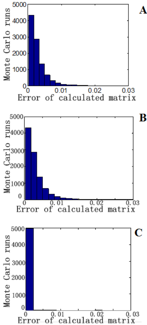
Figure 1. Error of the calculated matrix K_g represented by Frobenius norm. a) K_t assumed as upper triangular matrix; b) K_t assumed as lower triangular matrix; c) K_t assumed as diagonal matrix.
