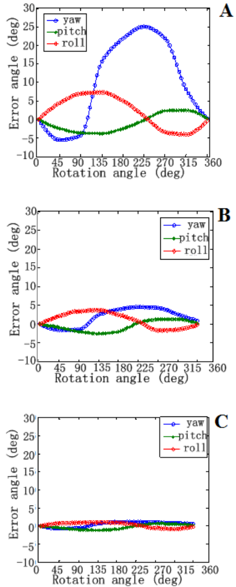
Figure 2. Accuracy of attitude using three calibration methods. A) None calibration; B) Ellipsoid fitting separate calibration; C) Proposed two-step calibration.
